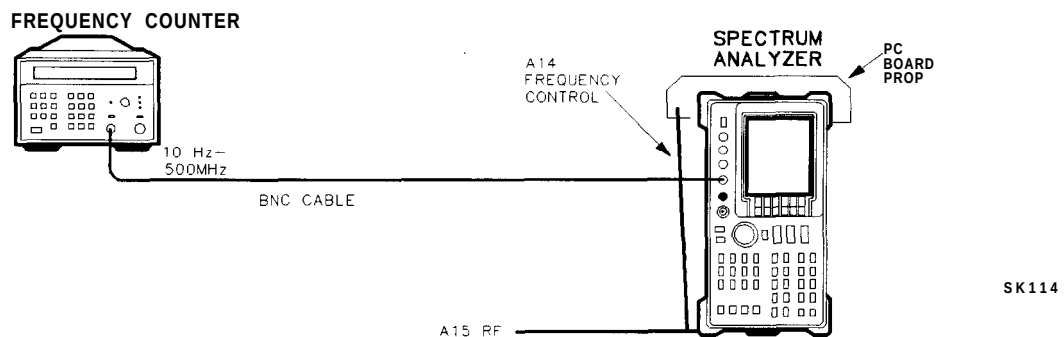
Figure 2-15. 10 MHz Frequency Reference Adjustment Setup
