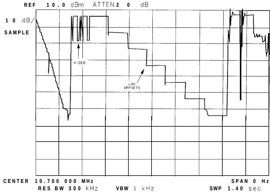
Figure 8-7. Detailed IF Adjust Signature (4)
