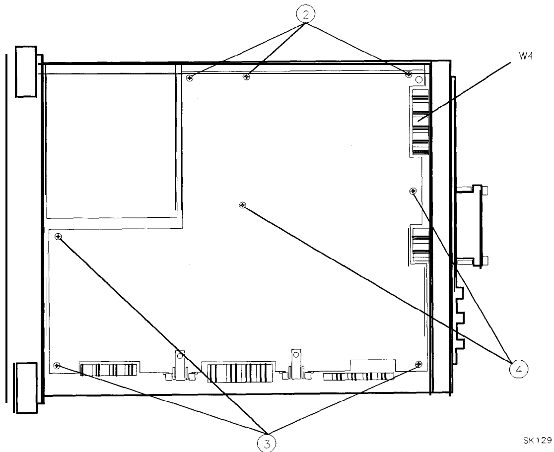
Figure 3-7. A2, A3, A4, and A5 Assembly Removal
