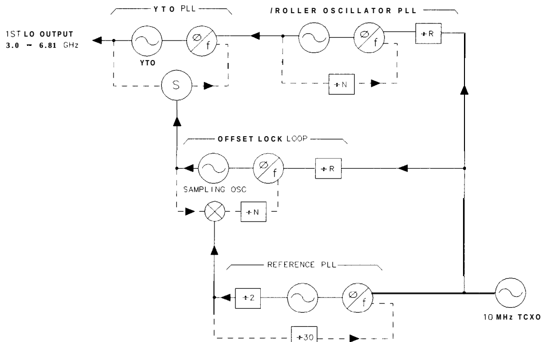
Figure 6-5. Phase Lock Loops
