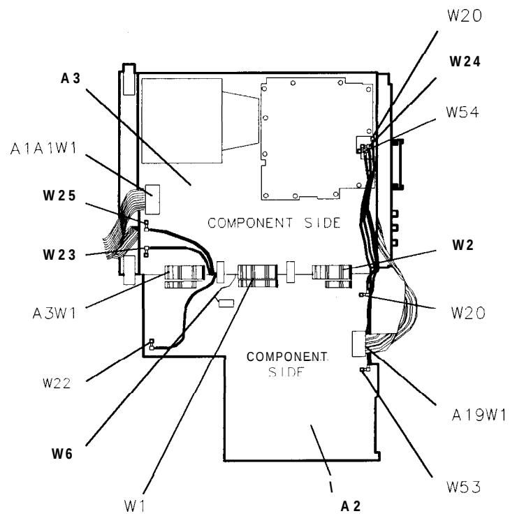
Figure 5-1. Hinged Assemblies
