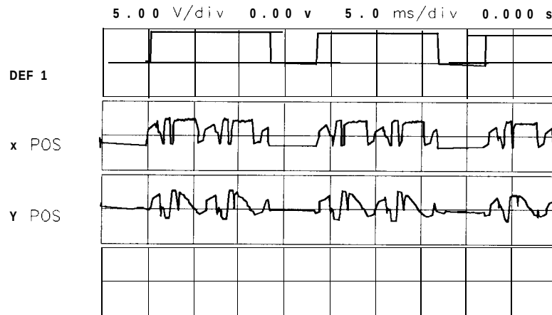
Figure 9-11. DEF1 Synchronization
