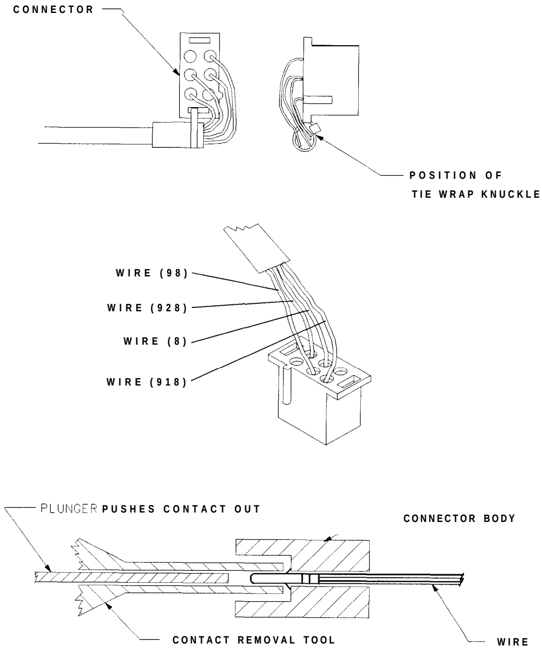
Figure 3-26. W3 Cable Connector
