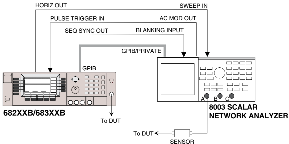
Figure 7-4. 682XXB/683XXB to 8003 SNA Connections
