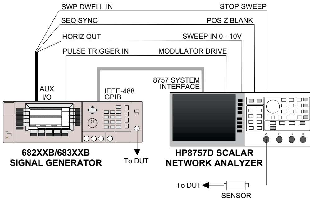
Figure 7-5. 682XXB/683XXB to HP8757D SNA Connections
