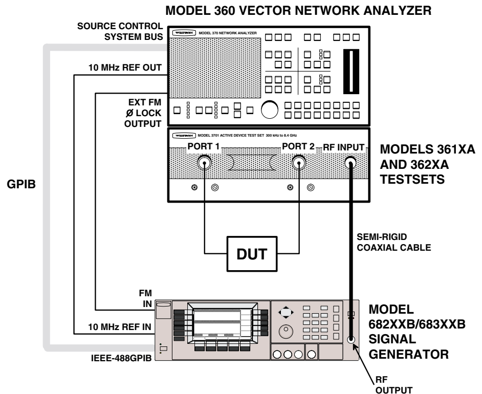
Figure 7-3. 682XXB/683XXB to 360B VNA Connections
