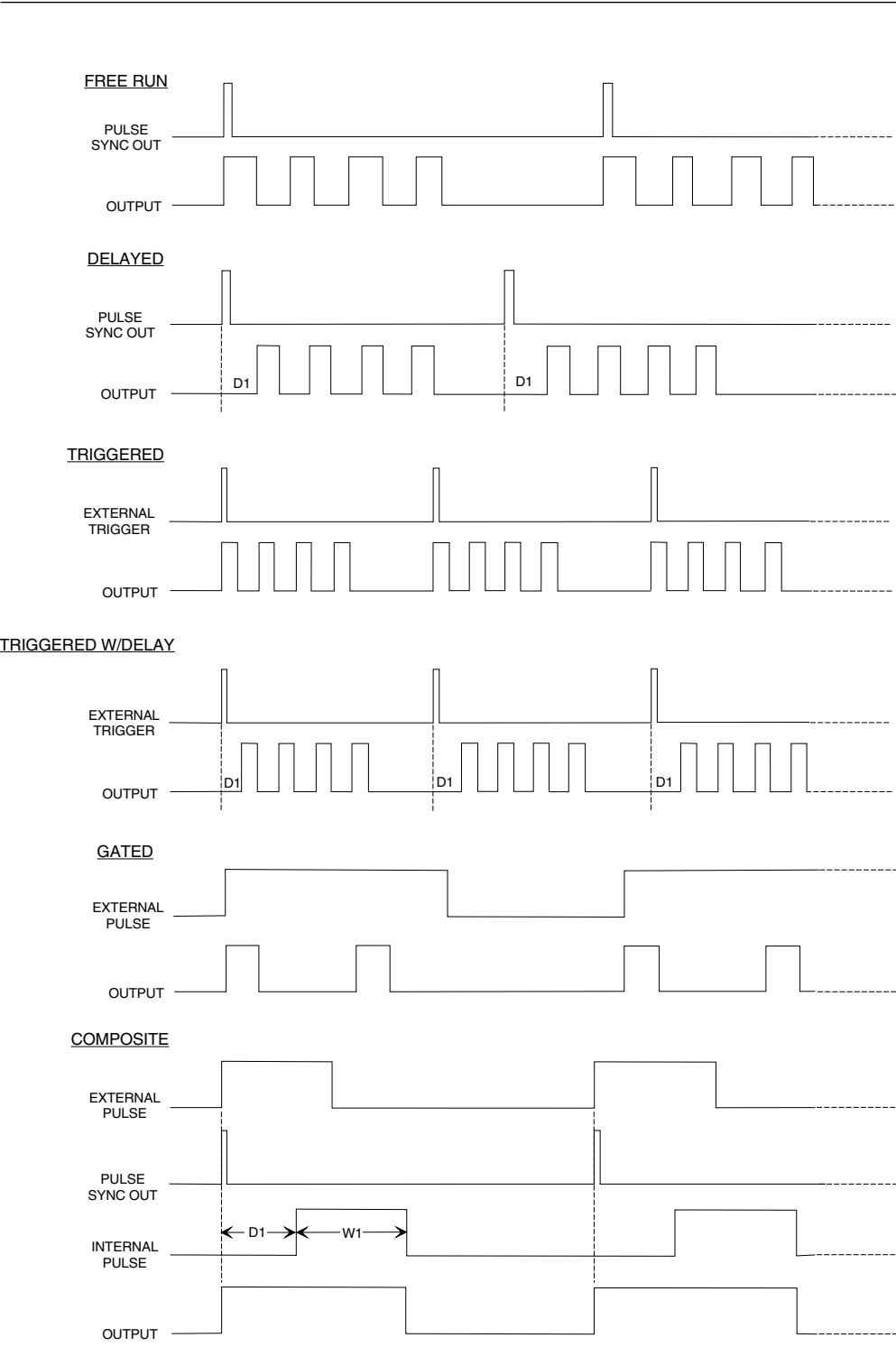
Figure 3-5. Pulse Modulation Triggering Modes
