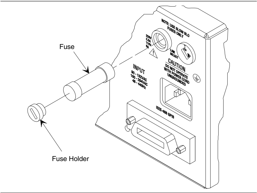
Figure 6-1. Replacing the Line Fuse
