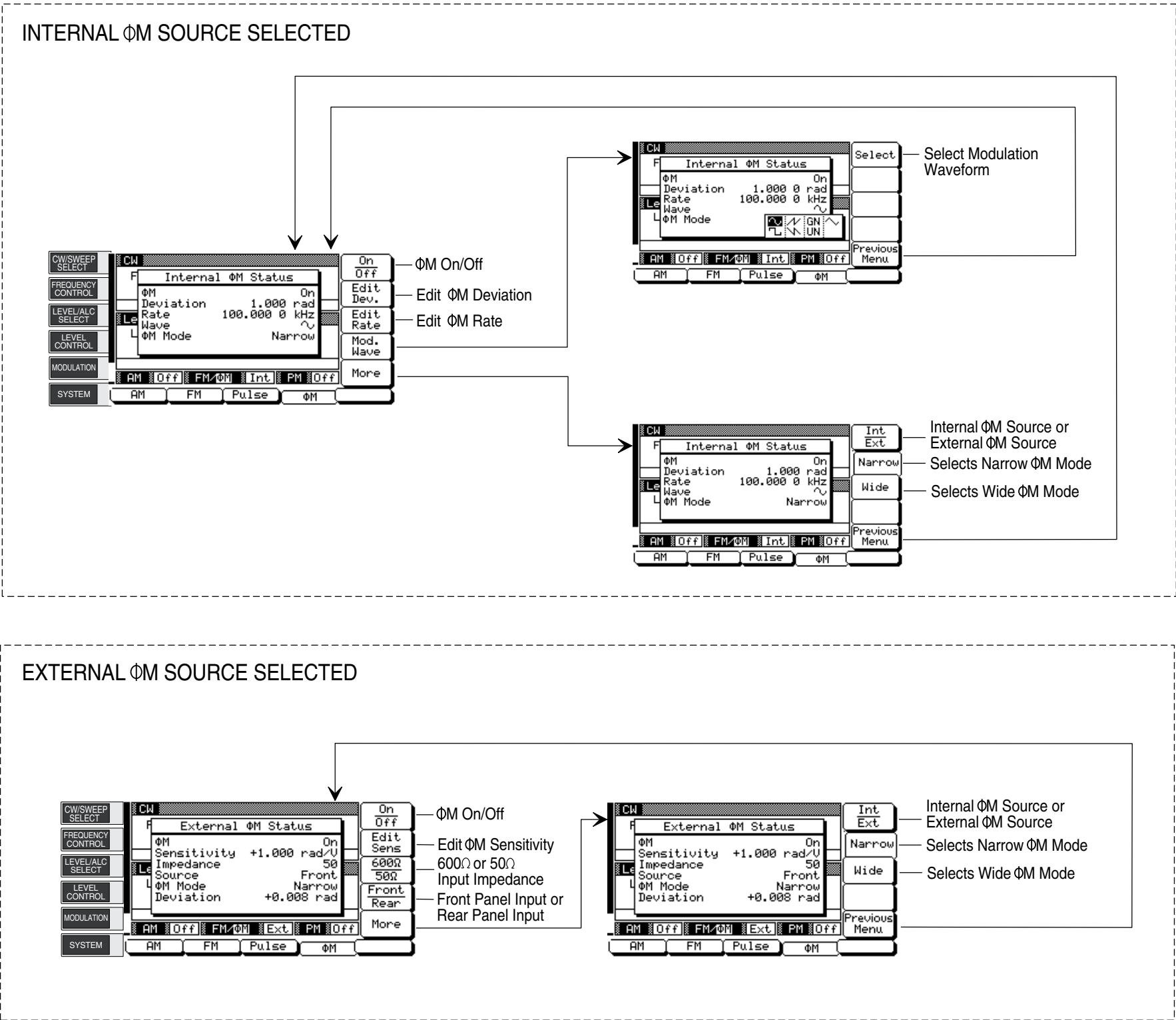
Figure 4-12. Phase Modulation Mode (Option 6) Menu Map
