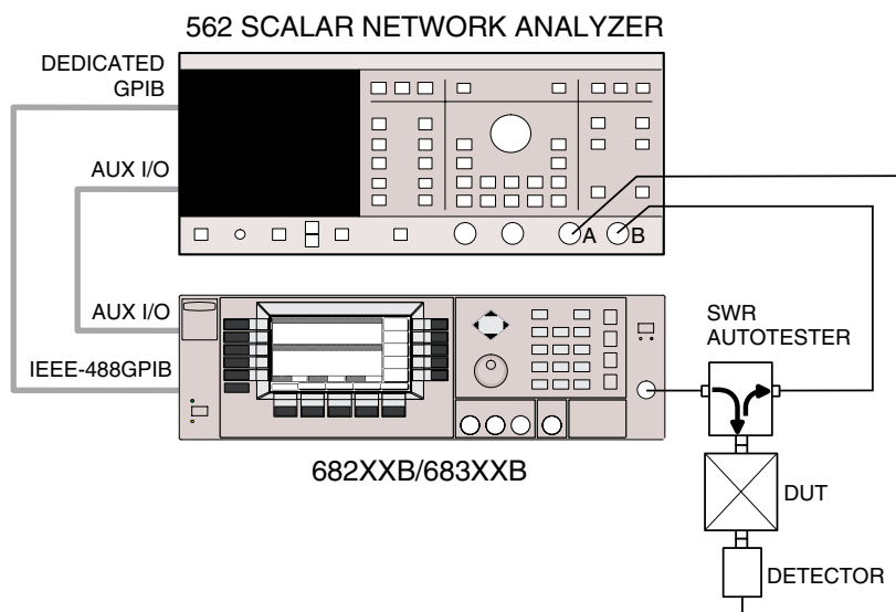
Figure 7-2. 682XXB/683XXB to 562 SNA Connections
