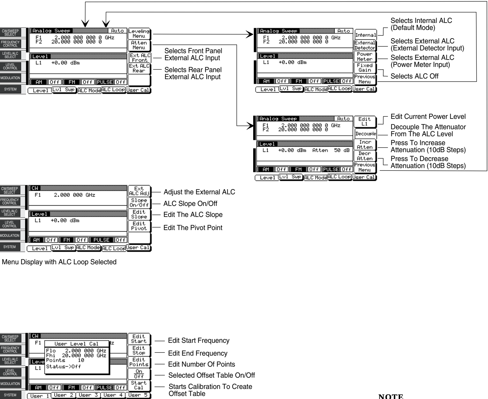
* Menu Display with User Cal Selected
