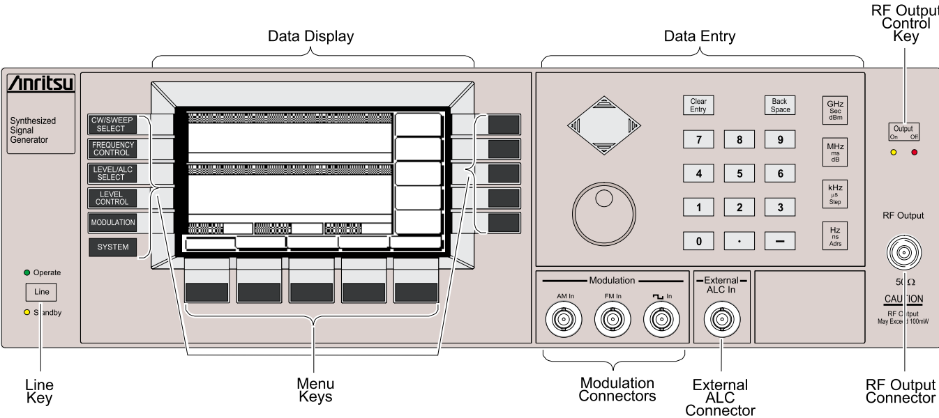
Figure 3-1. Front Panel, 682XXB/683XXB Synthesized Signal Generator
