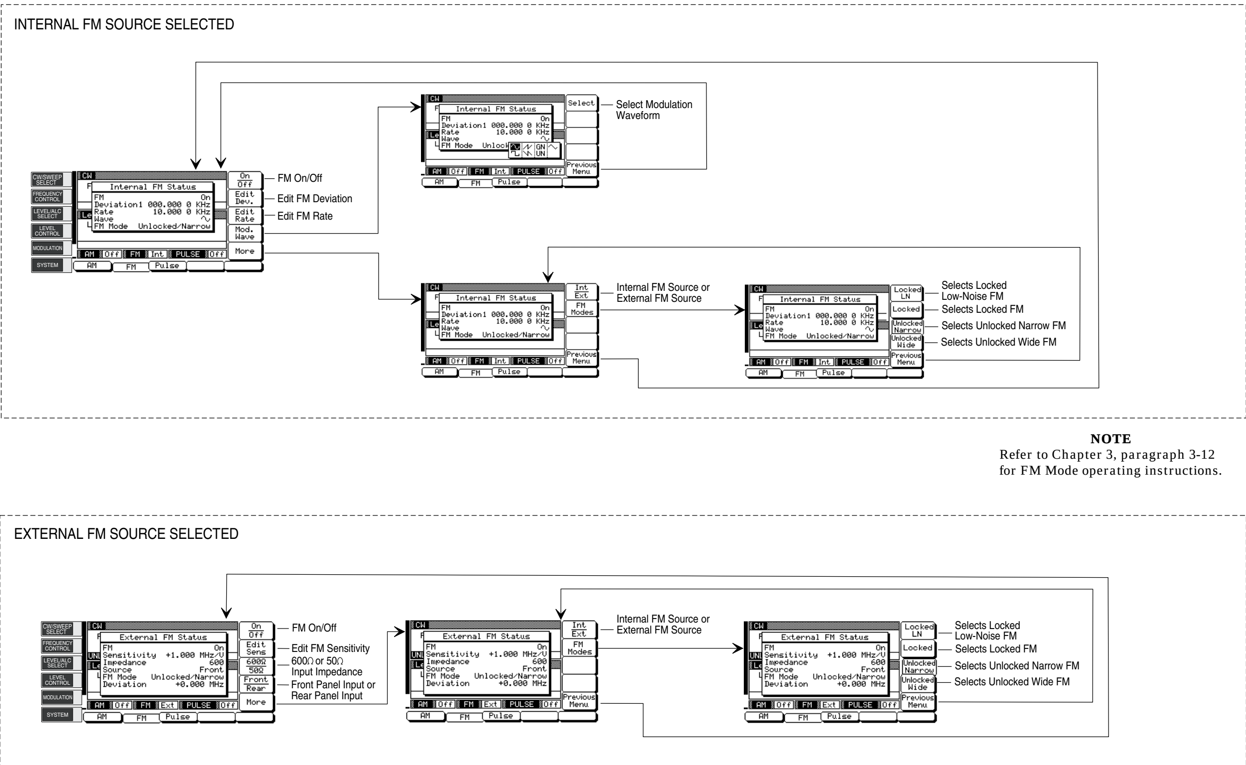
Figure 4-11. Frequency Modulation Mode Menu Map
