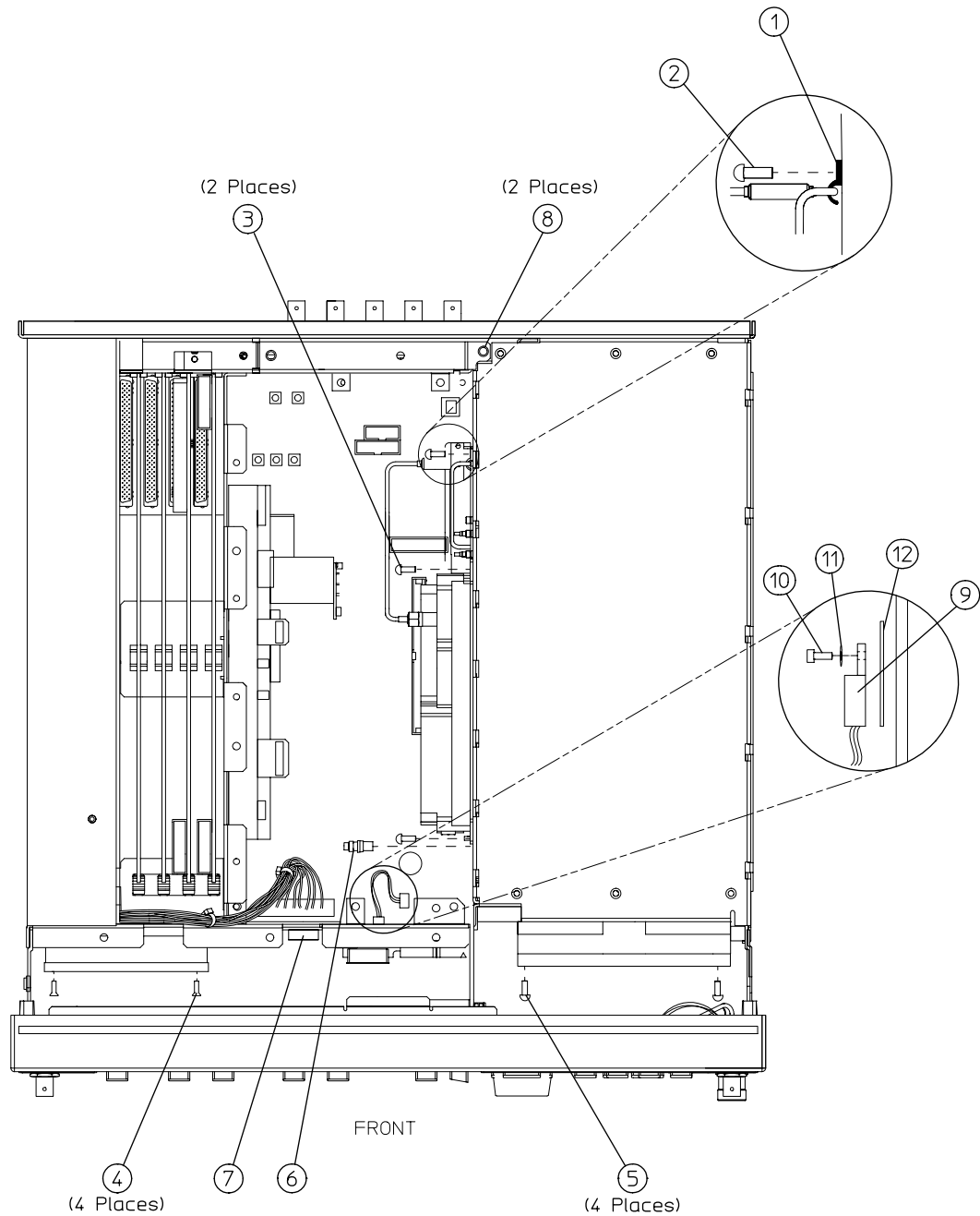
Figure 4-18 Top View
