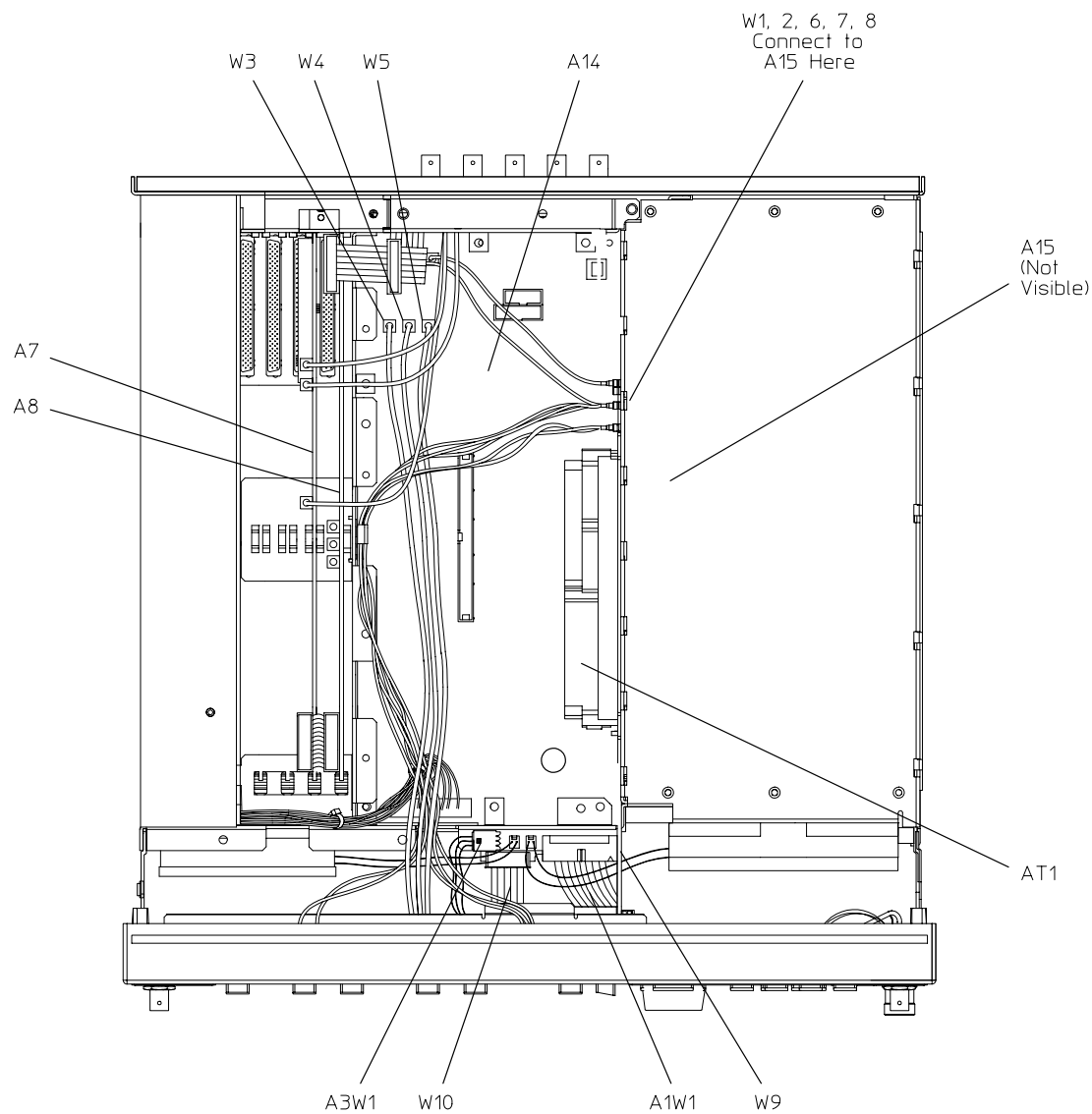
Figure 5-37 Front Panel (1 of 2)
