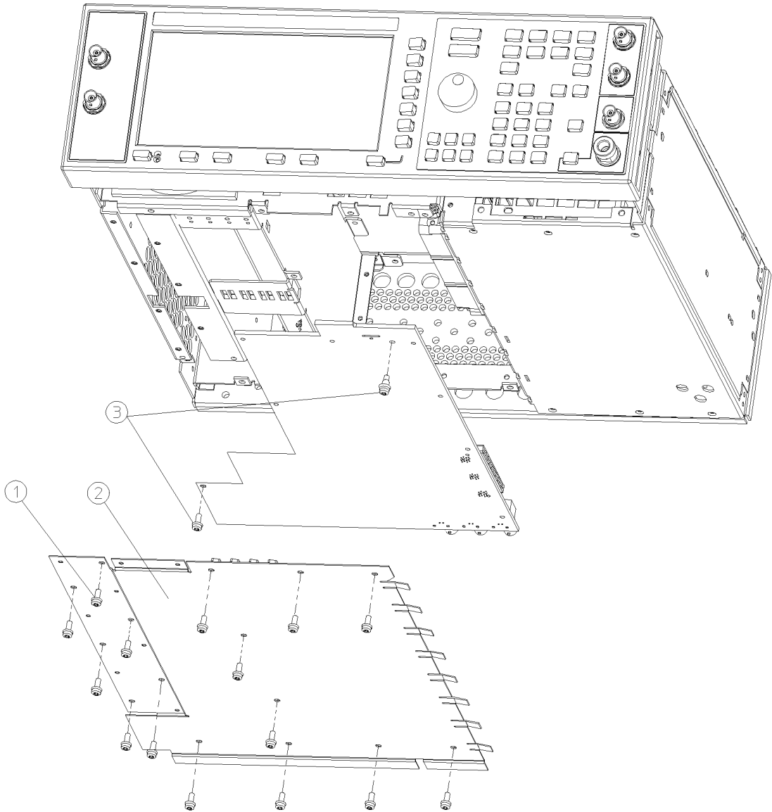
Figure 3-37 Motherboard and Bottom-Side Hardware
