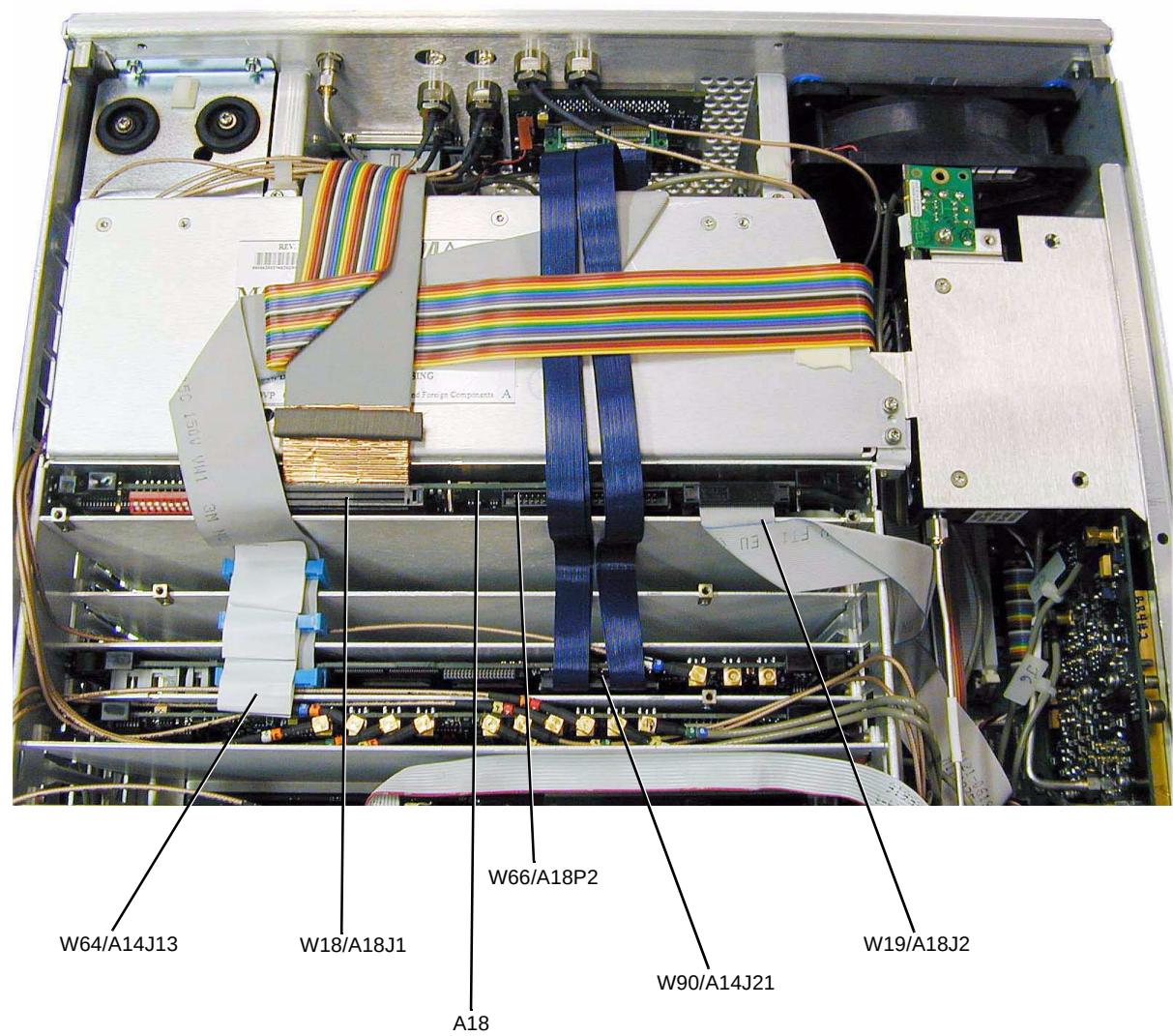
Figure 2-17 A18 CPU
