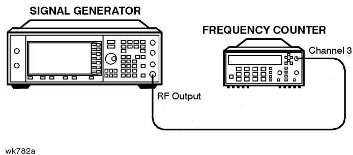
Figure 5-20 DCFM Calibration Setup
