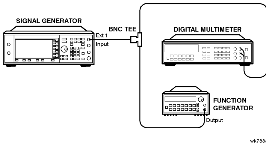
Figure 5-22 External Input Peak Detector Calibration Setup
