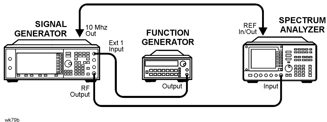
Figure 5-19 FM/PM YO Freq. Compensation Setup
