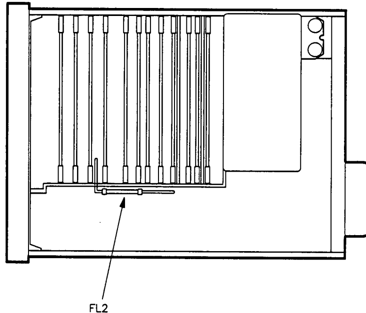
Figure 3-7. FL2 Location
