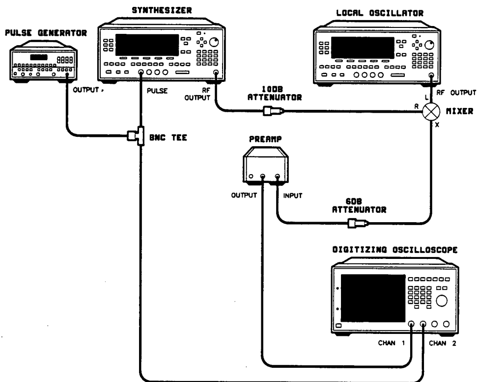
Figure 2-16. Pulse Performance Test Setup <20 GHz
