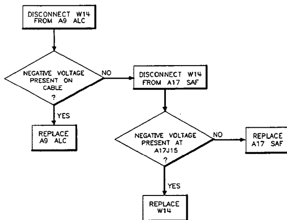
Troubleshooting Flow for A17 SAF
