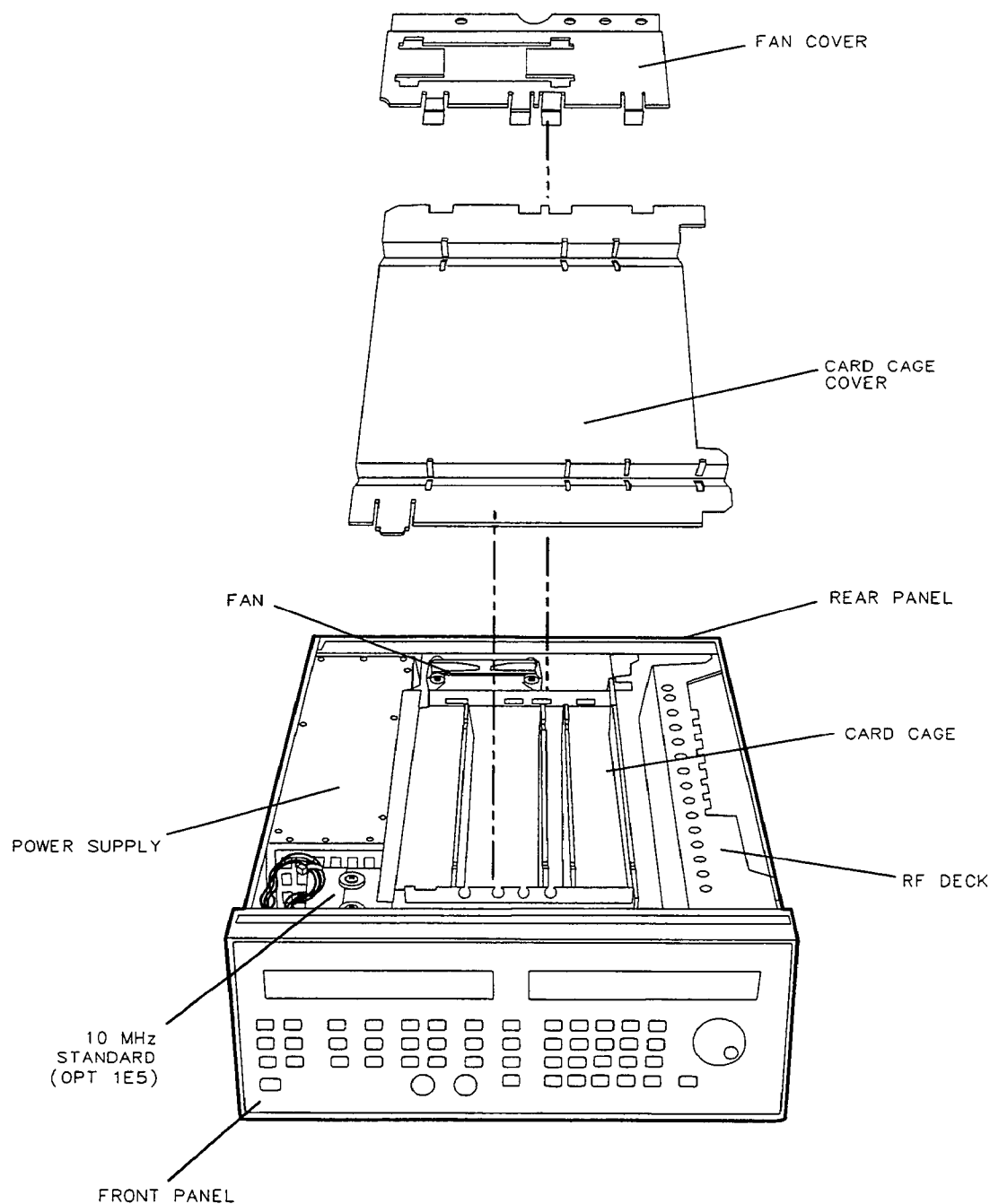
Figure 4-1. HP 83750 Overview
