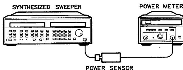
Figure 2-29. ALC Detector and Logger Adjustment Setup
