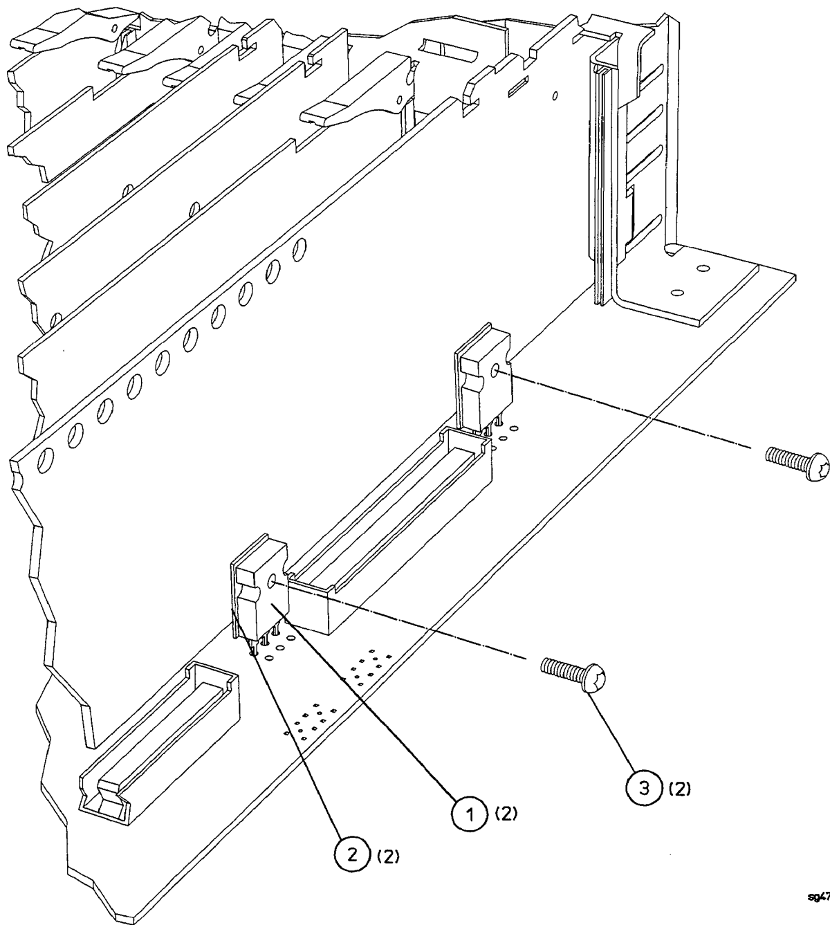
Figure 6-6. FET Assembly
