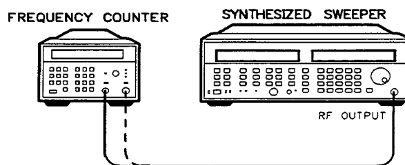
Figure 1-2. CW Frequency Accuracy Test Setup
