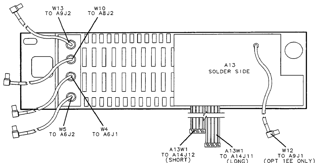
Figure 4-11. Rear Panel Cables
