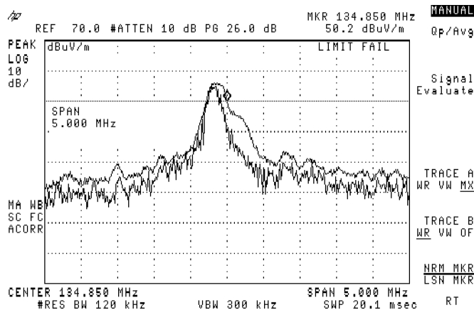
Figure 3-62. Trace A in Max Hold and Trace B in Clear Write
